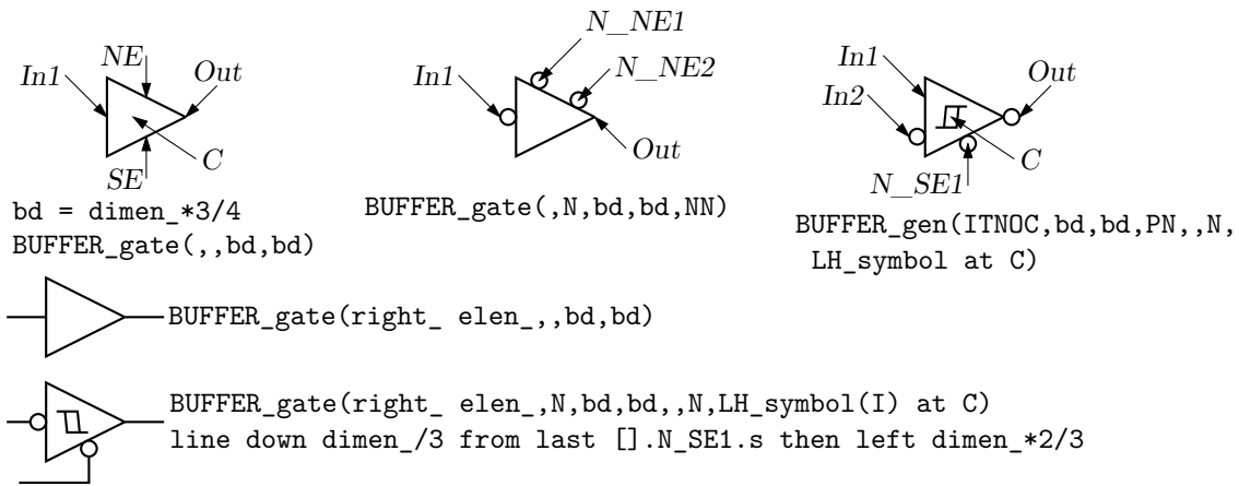
Figure 50: The BUFFER_gate and BUFFER_gen macros. The bottom two examples show how the gate can be drawn as a two-terminal macro but internal block locations must be referenced using last [] .
