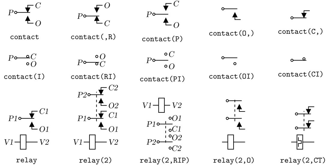
Figure 31: The contact(chars) and relay(poles, chars) macros (default direction right).
