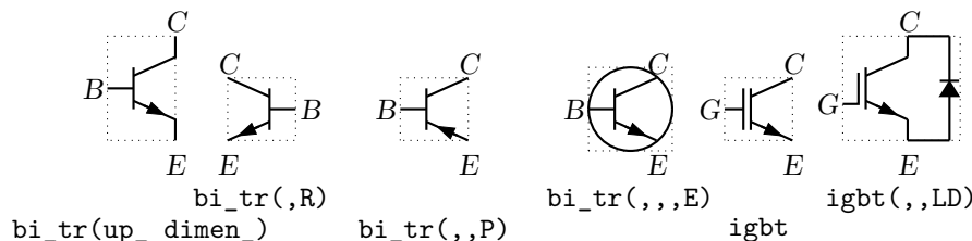
Figure 37: Bipolar transistor variants (current direction upward).
